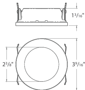
ED3-RFTL ROUND FIXED TRIMLESS Trimless Style for use with SAIC modules only.
