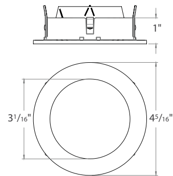
ED3-RFWW ROUND FIXED WALL WASH
