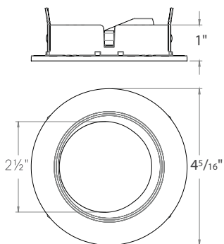
ED3-RAST ROUND ADJUSTABLE STANDARD TRIM Adjustable trim styles for use with adjustable SAIC models only.
