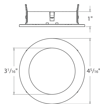
ED3-RFWL ROUND FIXED WET LOCATION
