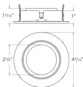
ED3-RFST ROUND FIXED STANDARD TRIM
