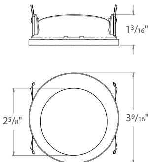
ED3-RATL ROUND ADJUSTABLE TRIMLESS Adjustable trim styles for use with adjustable AIC and SAIC models only.
